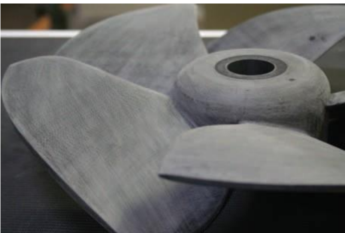
Fan prototype produced with FDM and sanded with an orbital sander
